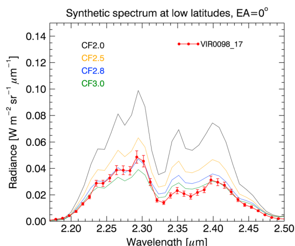
Figure 8. Comparison between synthetic spectra and an observed spectrum at the 2.3\mu\text{m} atmospheric window. The observation is taken from VIRTIS-M-IR on board Venus Express (orbit #0098 and cube #17). The observed spectrum is an average at low latitudes with less than 5^\circ emission angle at night side.
