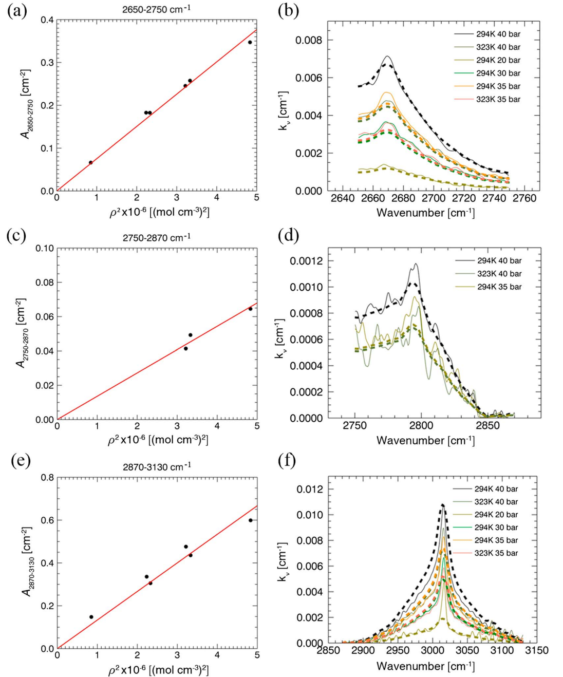
Figure 4. CO 2 CIA from laboratory experiments [Stefani et al., 2013]. (a, c, and e) Band integrated intensities as a function of density square. Linear fits are shown as red solid lines. (b, d, and f) The measured absorption coefficients at different pressures and temperatures (solid lines) and input data in our model calculation (dashed lines).
