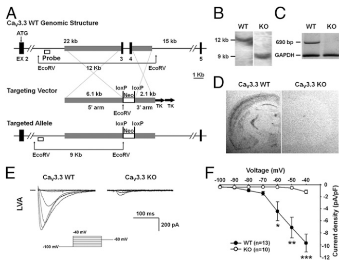
Fig. 1. Targeted disruption of the mouse \text{Ca}_v3.3 gene and decreased T-type current in \text{Ca}_v3.3 KO. (A) Schematic representations of the wild-type \text{Ca}_v3.3 allele, targeting vector, and mutant allele. Exons were represented by black boxes. Exon3 and exon4 were designed to be deleted to generate the mutant allele. (B) Southern blot analysis of genomic DNA isolated from tails of wild-type (WT) and homozygous KO mice. The restriction enzymes and probes used are shown in A. The 12 kb segment corresponds to the wild allele; the 9 kb, the targeted allele. (C) RT-PCR analysis was performed with mRNA derived from pooled samples of wild-type or the \text{Ca}_v3.3 mutant whole brain. PCR primers for RT-PCR were exon3–7. The 690 bp band indicates the PCR product of the wild type, whereas \text{Ca}_v3.3 mutant displays no band. (D) Quantitative analysis of the expression of the \text{Ca}_v3.3 mRNA with in situ hybridization. There is robust expression of \text{Ca}_v3.3 in the TRN of wild-type mouse but no expression in mutant TRN. Probes for in situ hybridization were exon3 and 4. (E) LVA \text{Ca}^{2+} currents were evoked by the depolarizing pulses ranging from -100 to -40 mV in wild-type and \text{Ca}_v3.3^{-/-} neurons. (F) Current–voltage relationship displayed a significant reduction in the peak current density in \text{Ca}_v3.3^{-/-} (open circle) compared with wild type (closed circle). Data are represented as mean \pm SEM; * P < 0.05 , ** P < 0.01 , *** P < 0.001 ; two-tailed t test.
