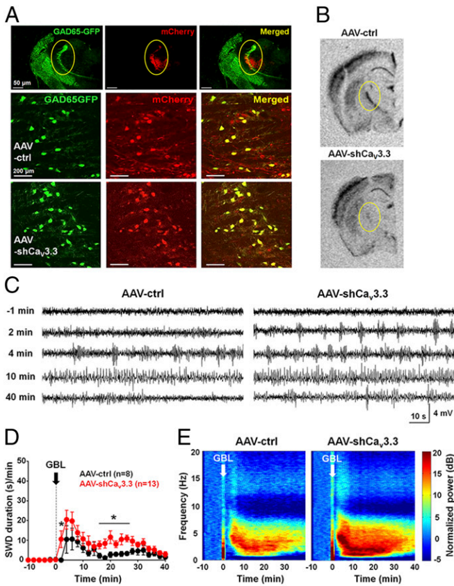
Fig. 3. Enhanced susceptibility to GBL-induced SWD after microinjection of AAV-shCa v 3.3 in the TRN of GAD65-GFP mice. (A) Confocal images showing expression of AAV-control and AAV-shCa v 3.3 (yellow circles indicate the TRN region in Top panels). Virus-infected neurons are colabeled with GFP (green, GAD65-GFP-positive neurons; red, AAV-control-infected neurons in Middle panel; and AAV-shCa v 3.3 in Bottom panel; yellow, merged). (B) Representative images of in situ hybridization ( Upper , AAV-control; Lower , AAV-shCa v 3.3). (C) EEG traces of AAV-control ( Left ) and AAV-shCa v 3.3 mice ( Right ) for 1 min before and various times after GBL injection. (D) SWD density calculated by total duration of SWD per min in AAV-control- (black circle) and AAV-shCa v 3.3- (red circle) injected mice. (E) Average EEG power spectrograms of AAV-control- and AAV-shCa v 3.3-injected mice during a 50-min recording. GBL was injected after 10 min of baseline recording. Data are represented as mean ± SEM, * P < 0.05.
